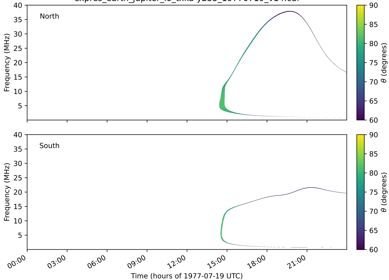
expres_earth_jupiter_io_txka-y235_19770719_v14.cdf
