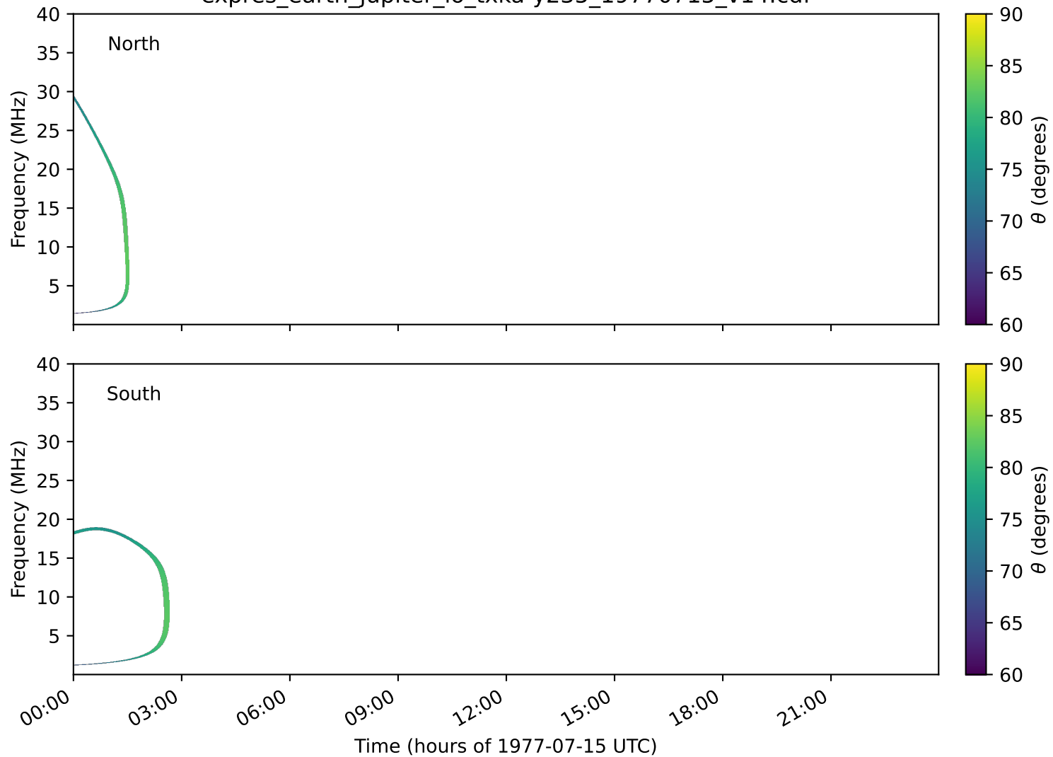
expres_earth_jupiter_io_txka-y235_19770715_v14.cdf
