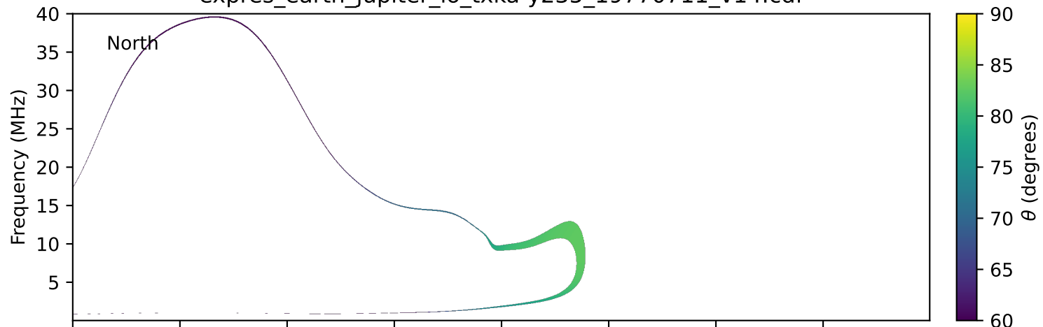
expres_earth_jupiter_io_txka-y235_19770711_v14.cdf
