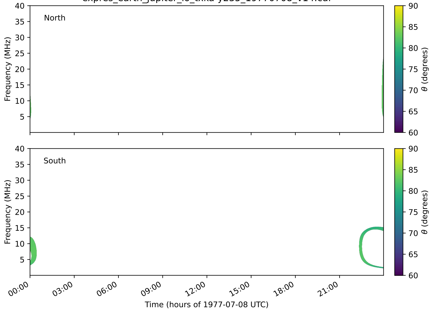
expres_earth_jupiter_io_txka-y235_19770708_v14.cdf
