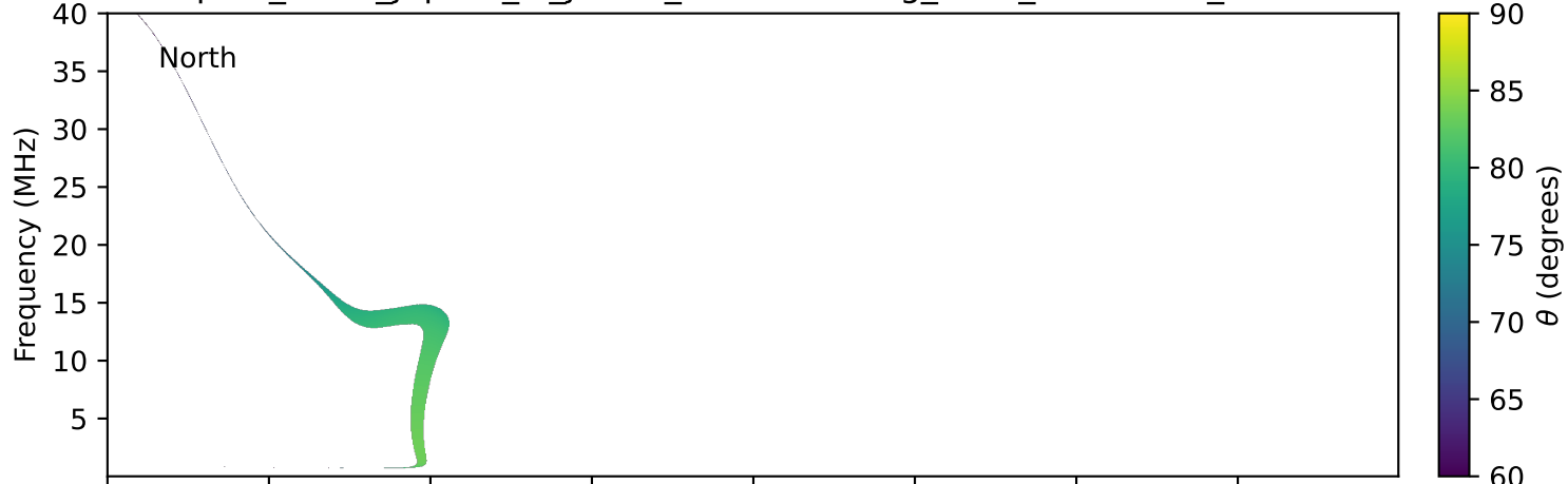
expres_earth_jupiter_io_jrm33_lossc-wid1deg_3kev_19770729_v11.cdf
