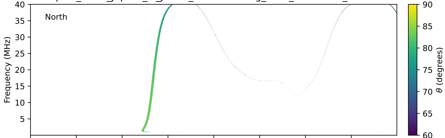
expres_earth_jupiter_io_jrm33_lossc-wid1deg_3kev_19770714_v11.cdf
