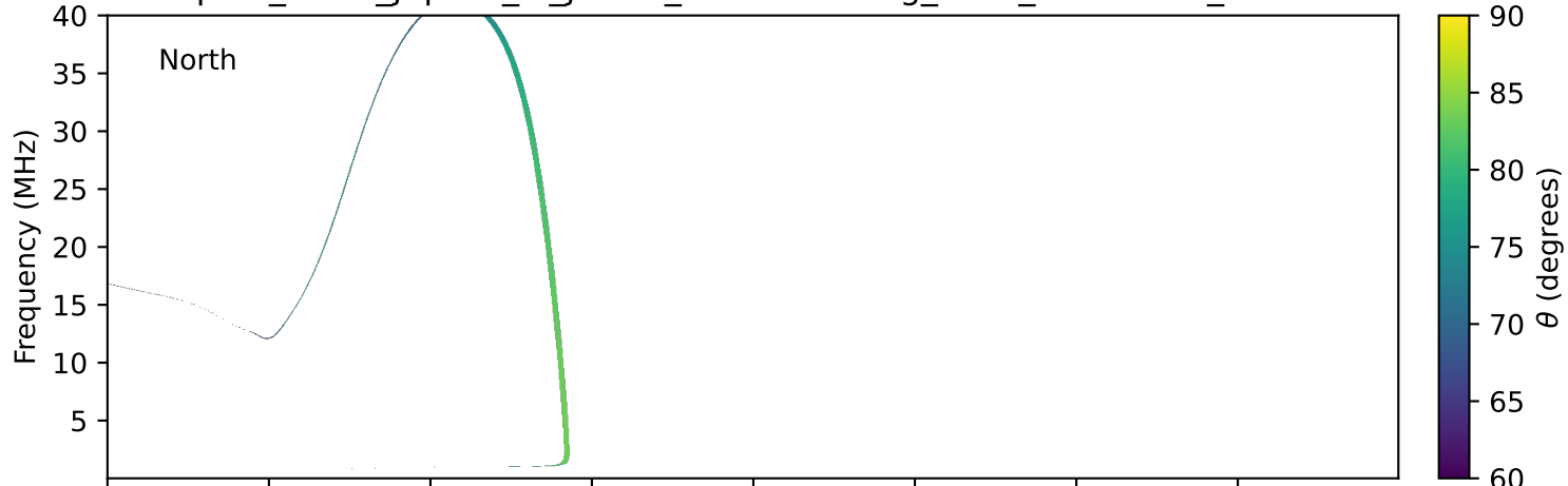
expres_earth_jupiter_io_jrm09_lossc-wid1deg_3kev_19770713_v11.cdf
