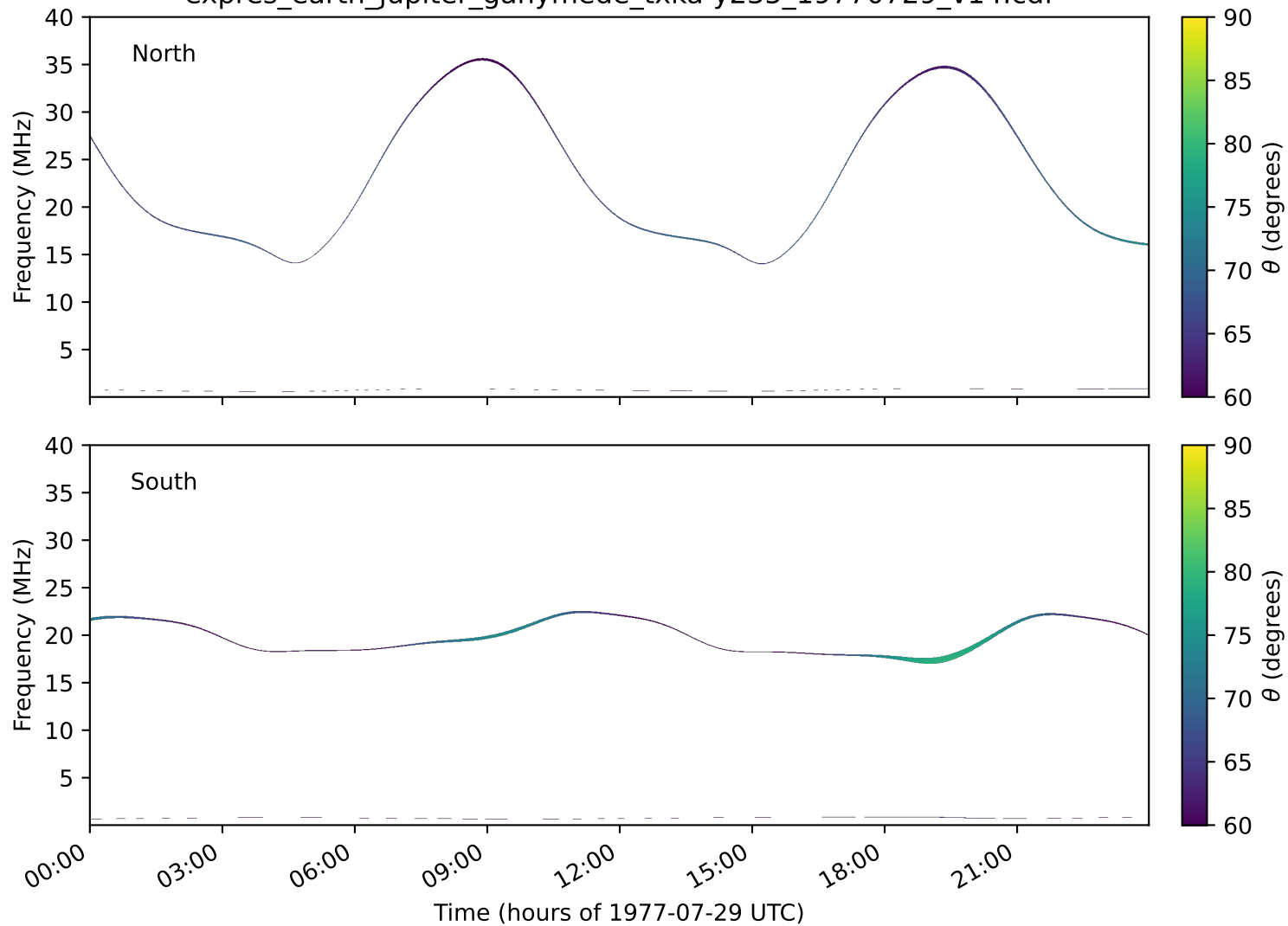
expres_earth_jupiter_ganymede_txka-y235_19770729_v14.cdf
