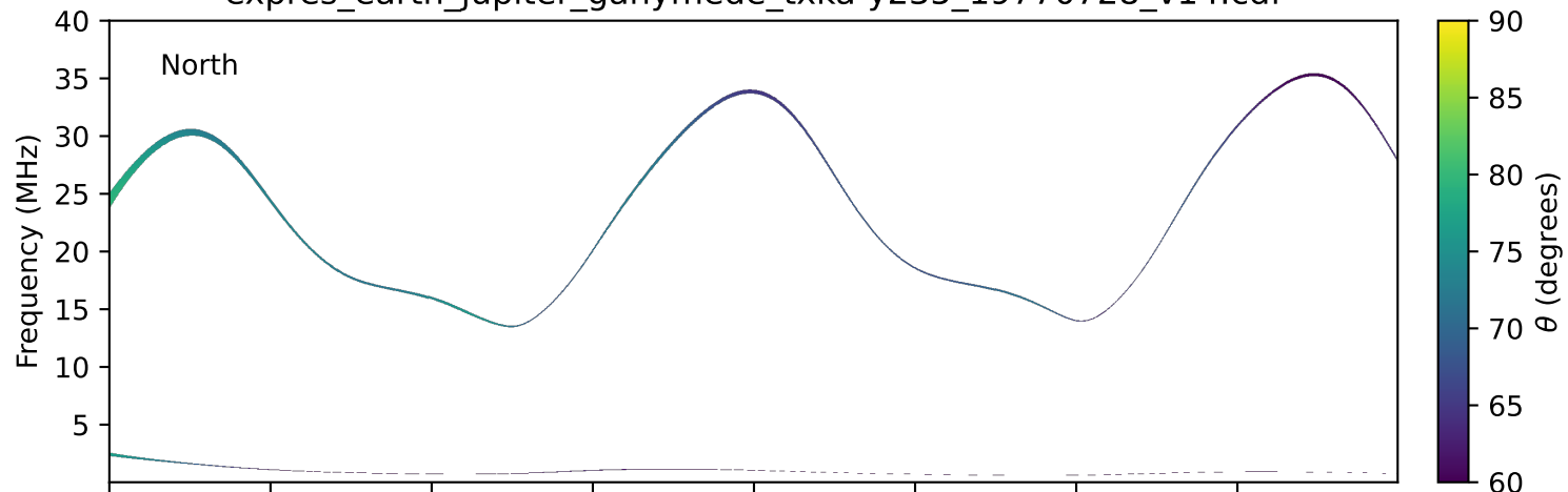
expres_earth_jupiter_ganymede_txka-y235_19770728_v14.cdf
