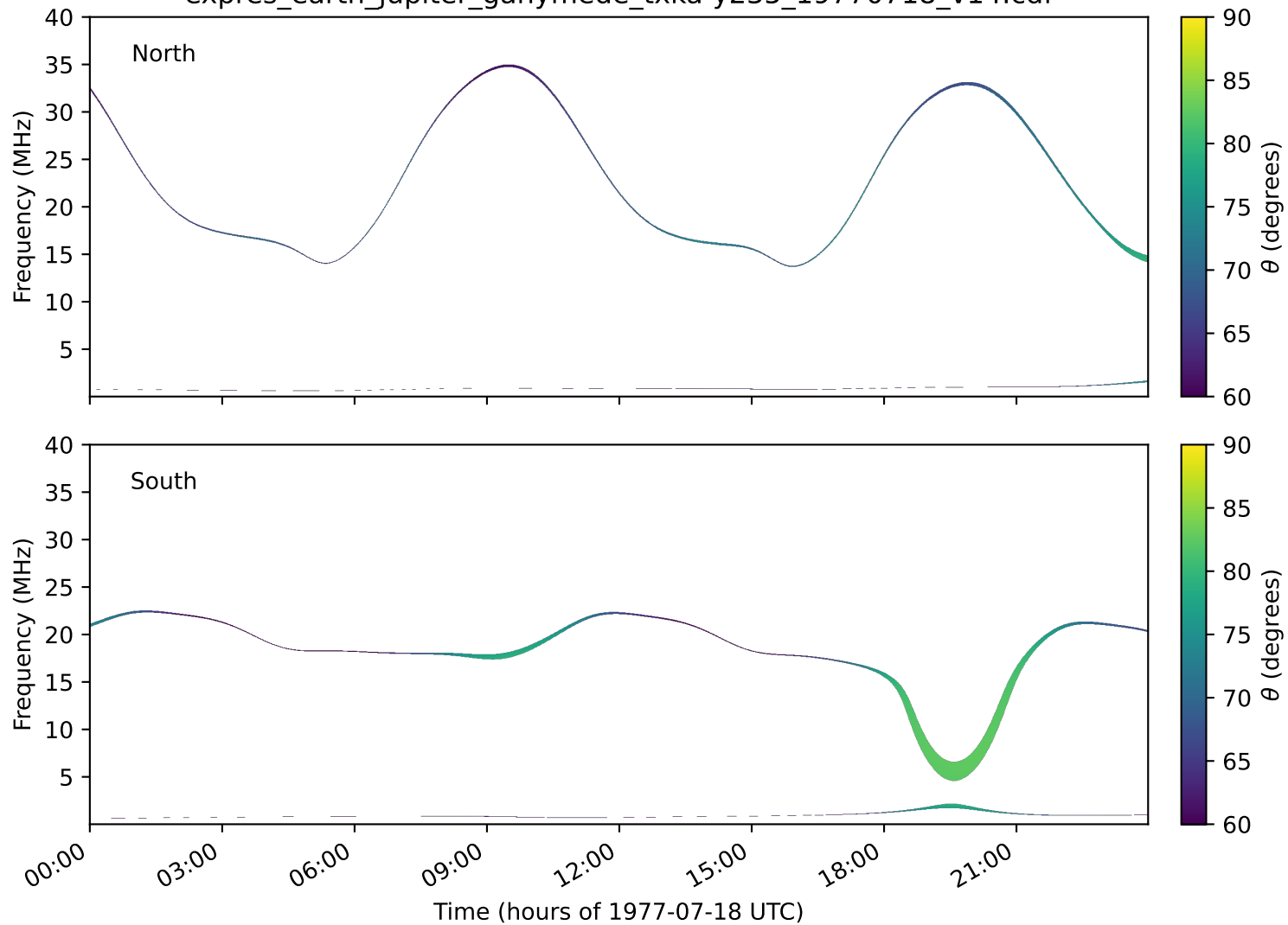
expres_earth_jupiter_ganymede_txka-y235_19770718_v14.cdf
