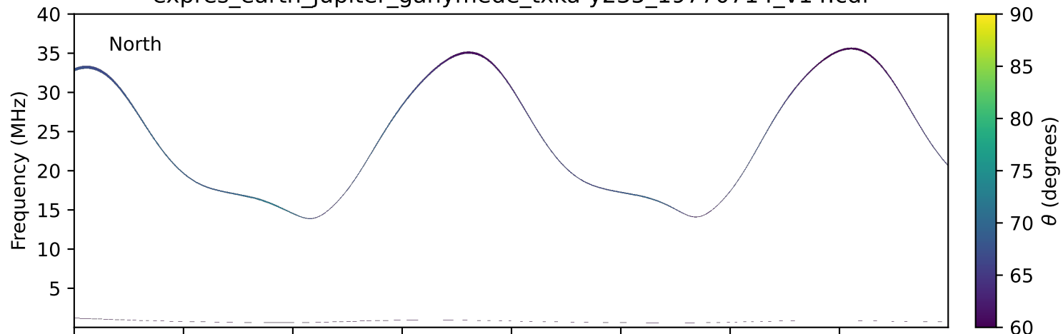
expres_earth_jupiter_ganymede_txka-y235_19770714_v14.cdf
