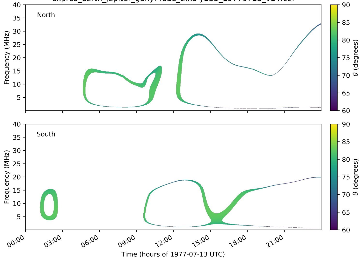
expres_earth_jupiter_ganymede_txka-y235_19770713_v14.cdf
