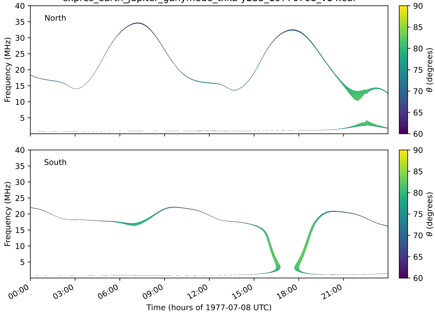
expres_earth_jupiter_ganymede_txka-y235_19770708_v14.cdf
