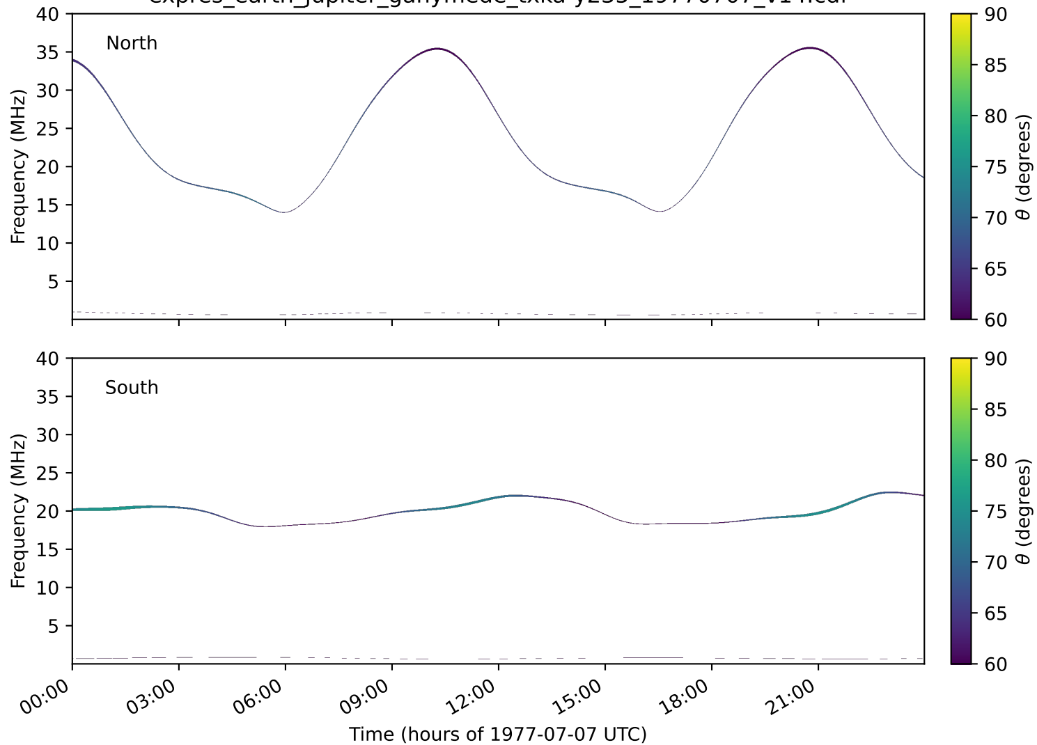
expres_earth_jupiter_ganymede_txka-y235_19770707_v14.cdf
