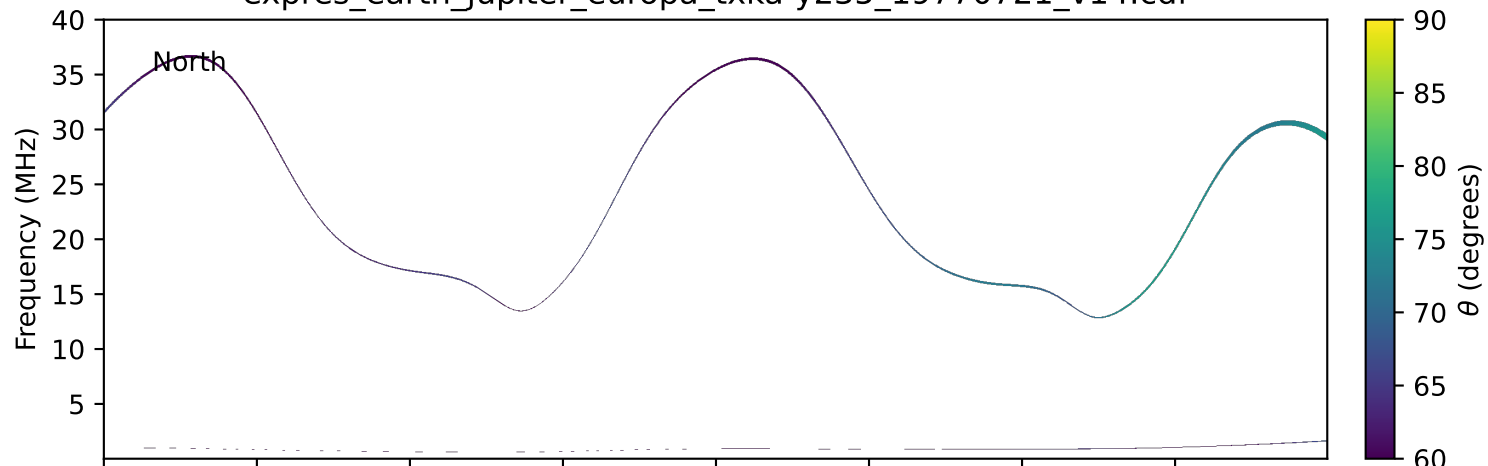
expres_earth_jupiter_europa_txka-y235_19770721_v14.cdf
