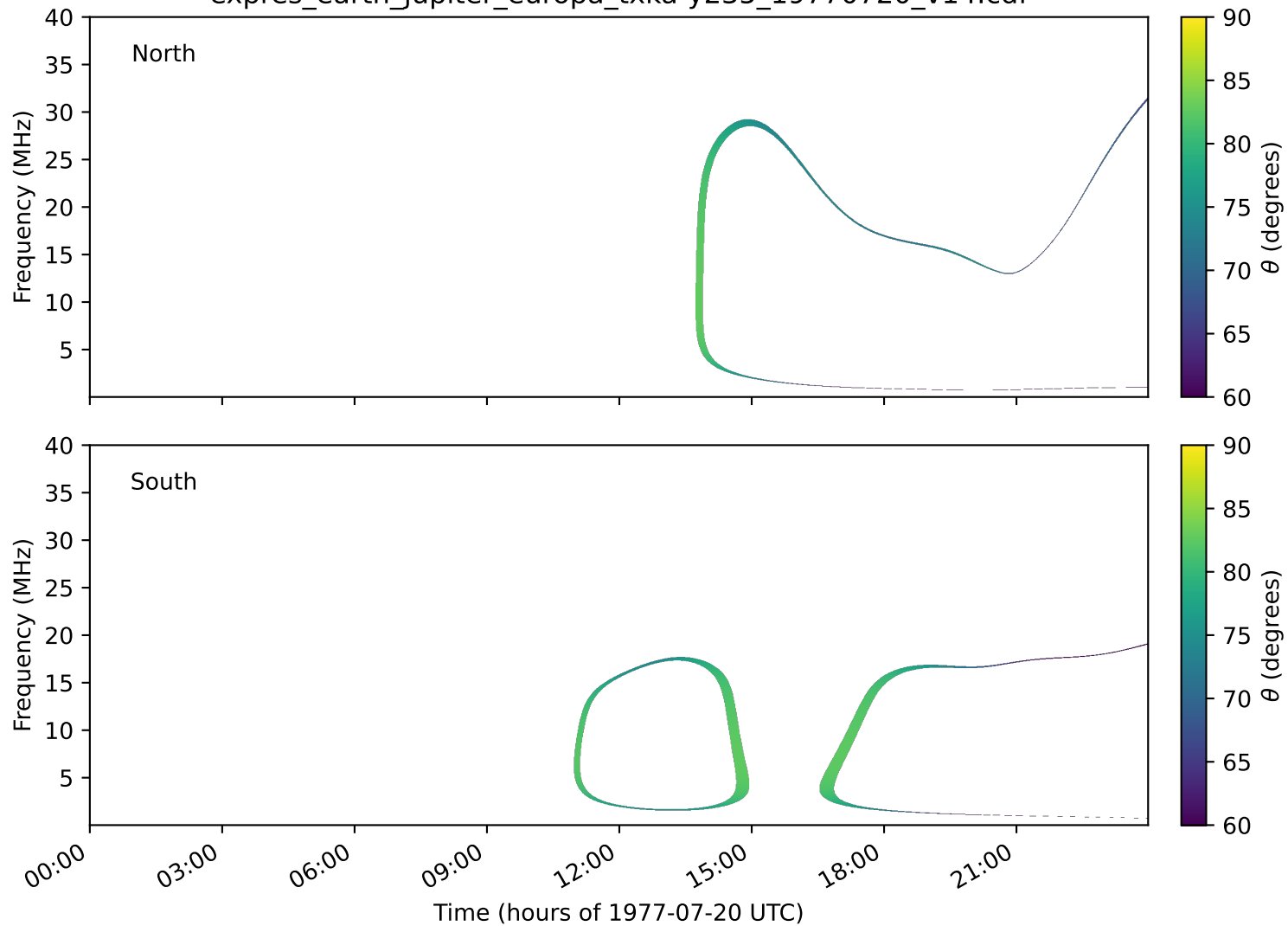
expres_earth_jupiter_europa_txka-y235_19770720_v14.cdf
