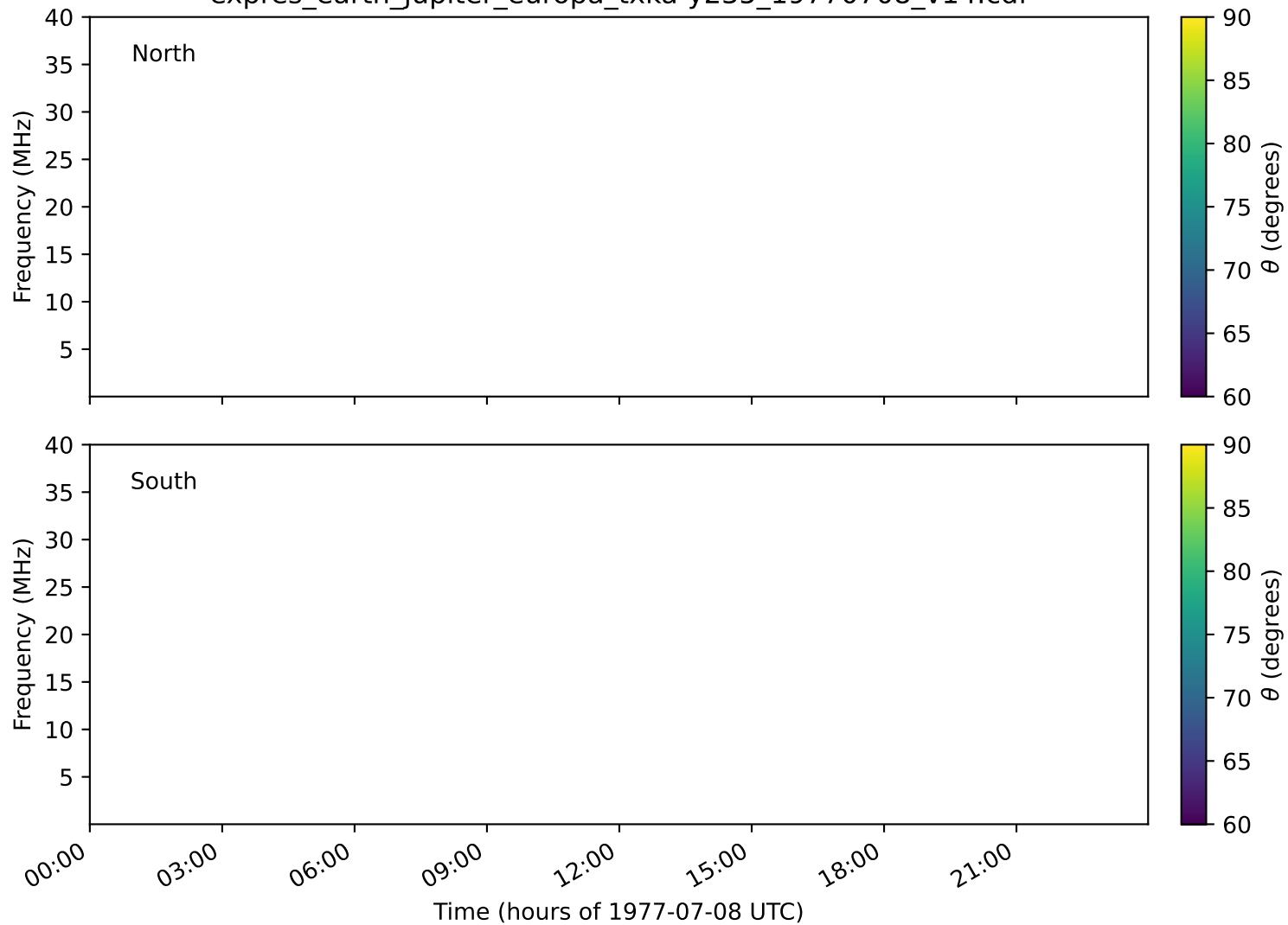
expres_earth_jupiter_europa_txka-y235_19770708_v14.cdf
