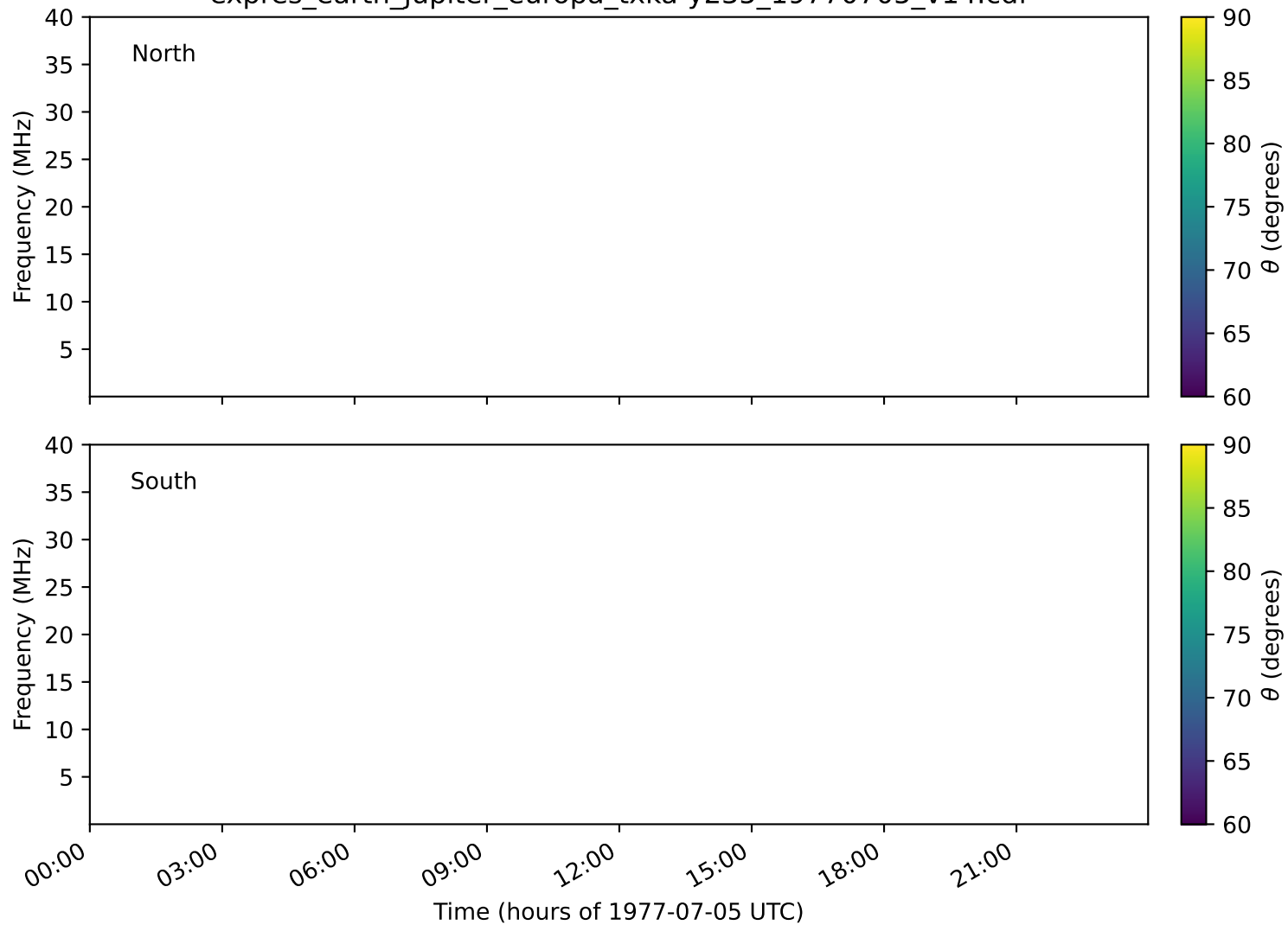
expres_earth_jupiter_europa_txka-y235_19770705_v14.cdf
