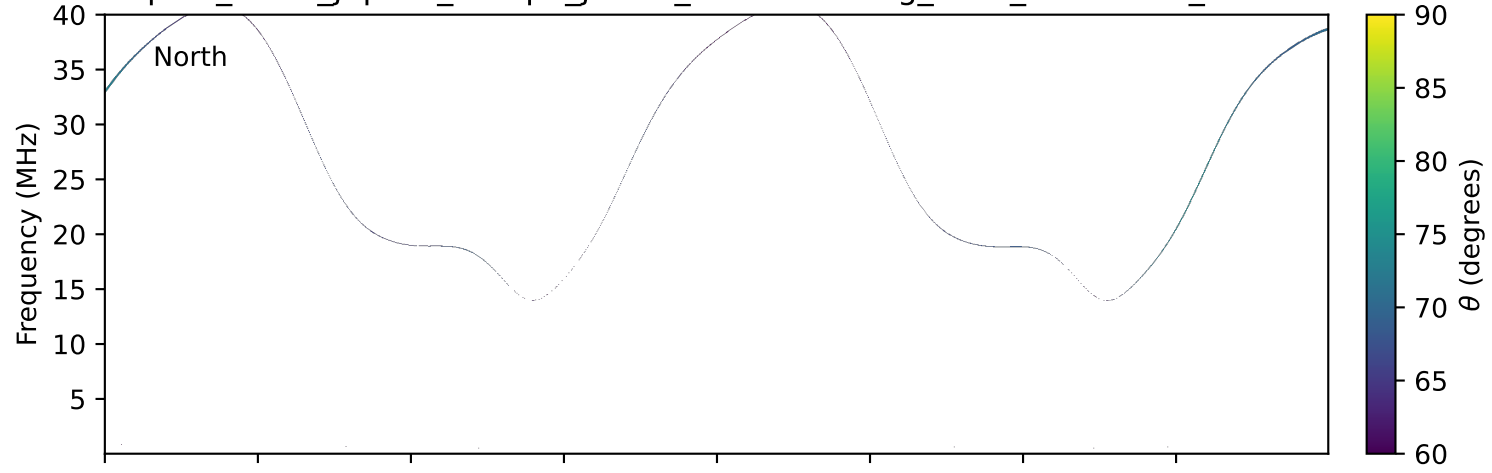
expres_earth_jupiter_europa_jrm33_lossc-wid1deg_3kev_19770728_v11.cdf
