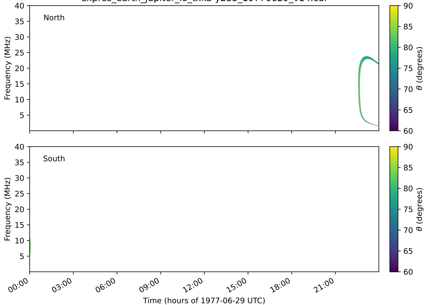
expres_earth_jupiter_io_txka-y235_19770629_v14.cdf
