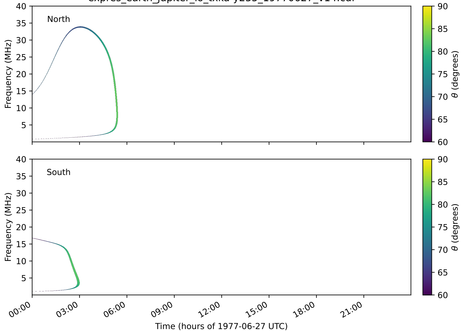
expres_earth_jupiter_io_txka-y235_19770627_v14.cdf
