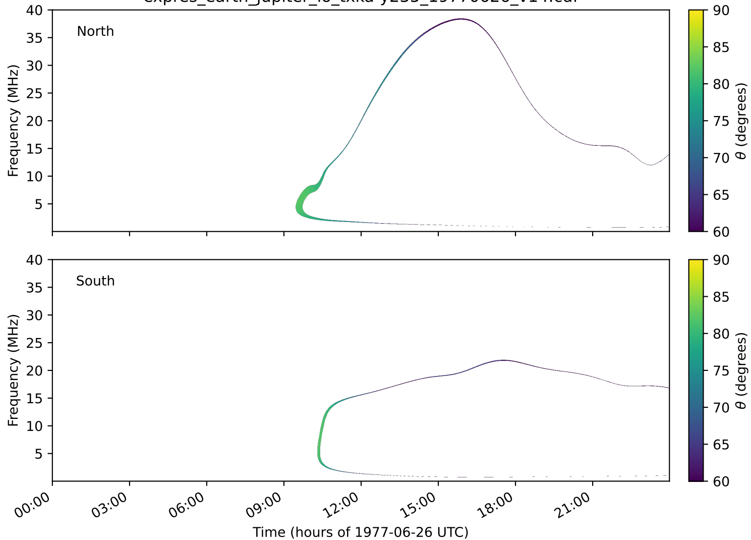
expres_earth_jupiter_io_txka-y235_19770626_v14.cdf
