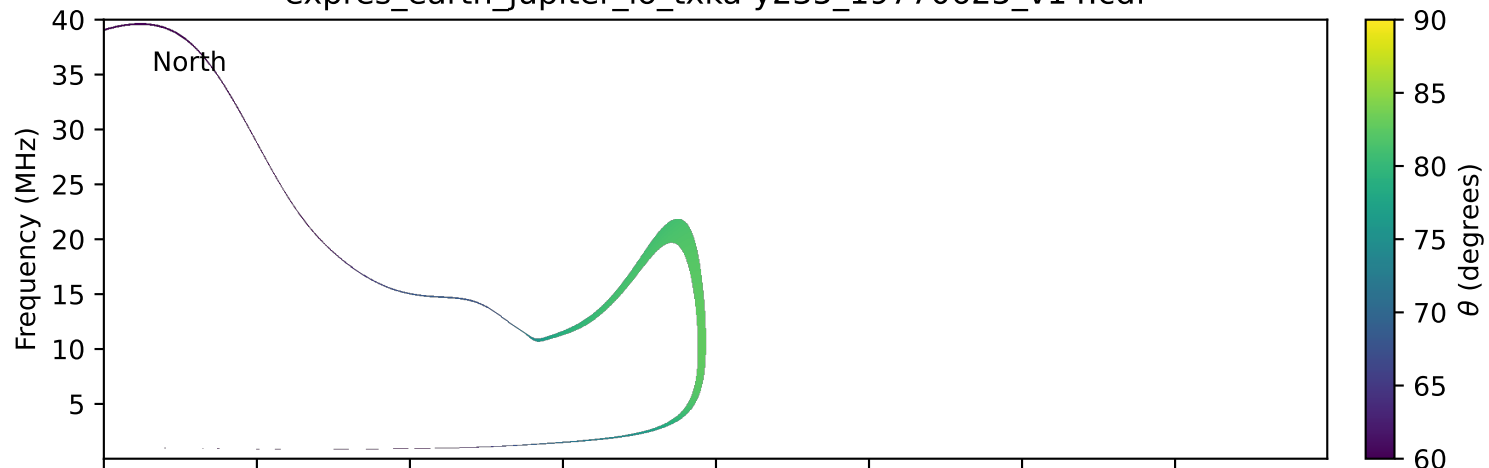
expres_earth_jupiter_io_txka-y235_19770625_v14.cdf
