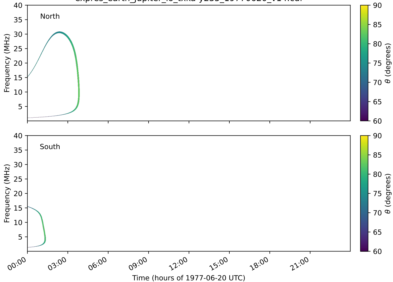
expres_earth_jupiter_io_txka-y235_19770620_v14.cdf
