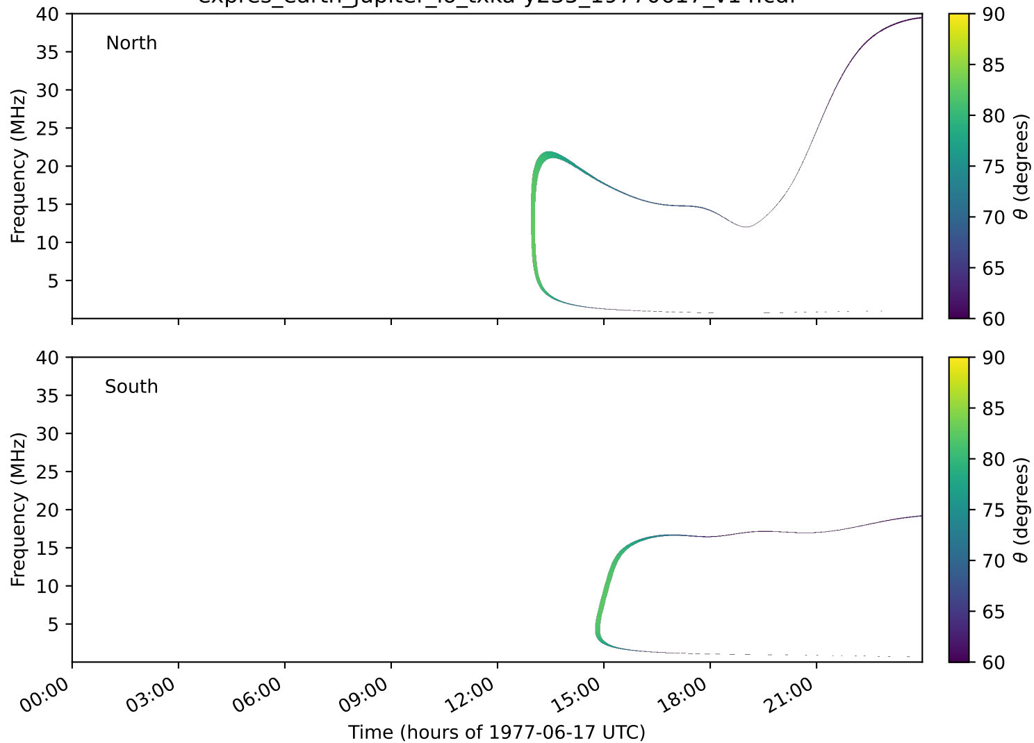
expres_earth_jupiter_io_txka-y235_19770617_v14.cdf
