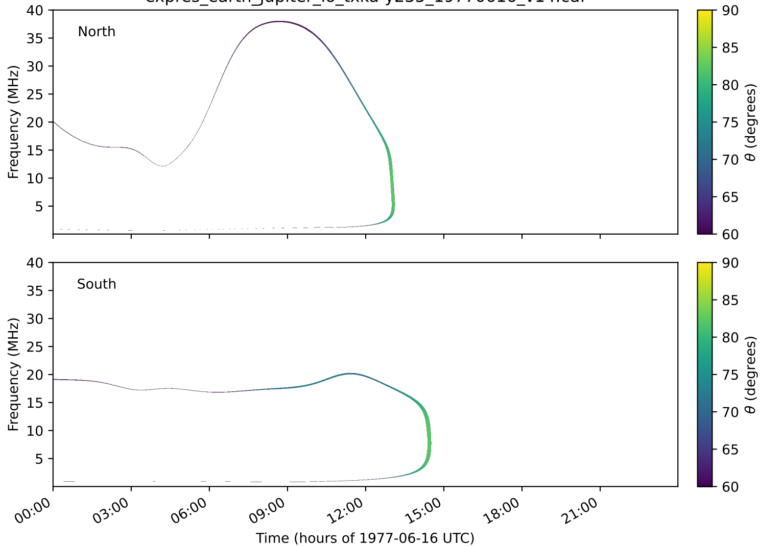
expres_earth_jupiter_io_txka-y235_19770616_v14.cdf
