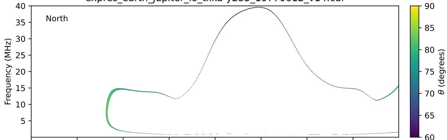
expres_earth_jupiter_io_txka-y235_19770612_v14.cdf
