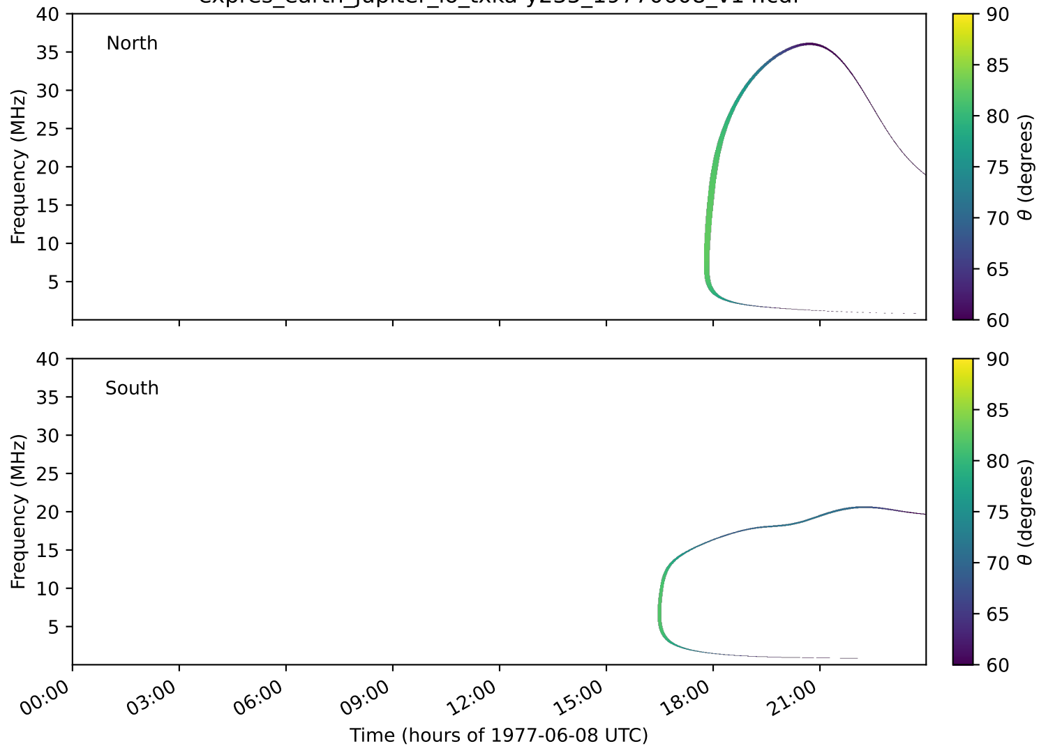
expres_earth_jupiter_io_txka-y235_19770608_v14.cdf
