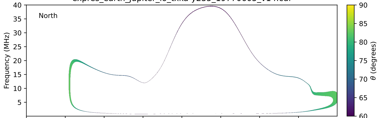
expres_earth_jupiter_io_txka-y235_19770605_v14.cdf
