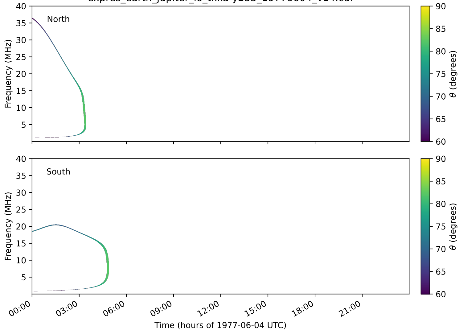
expres_earth_jupiter_io_txka-y235_19770604_v14.cdf
