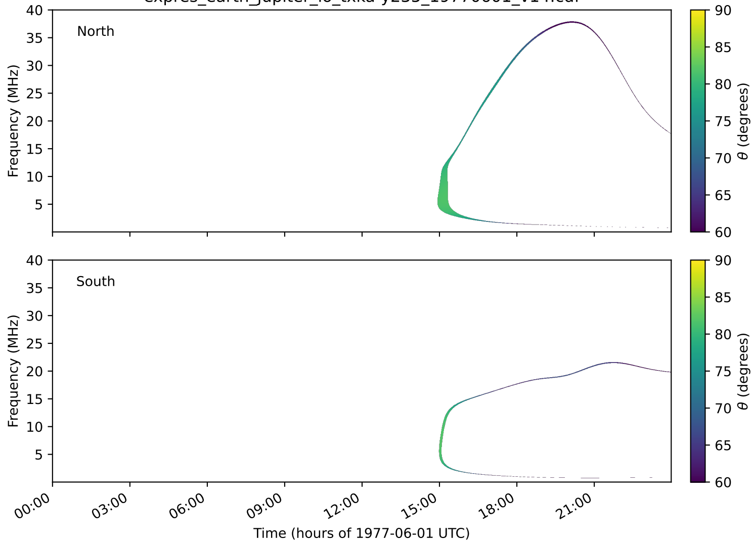
expres_earth_jupiter_io_txka-y235_19770601_v14.cdf
