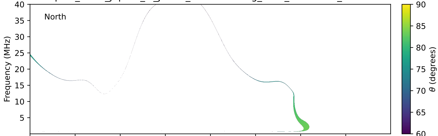
expres_earth_jupiter_io_jrm33_lossc-wid1deg_3kev_19770630_v11.cdf
