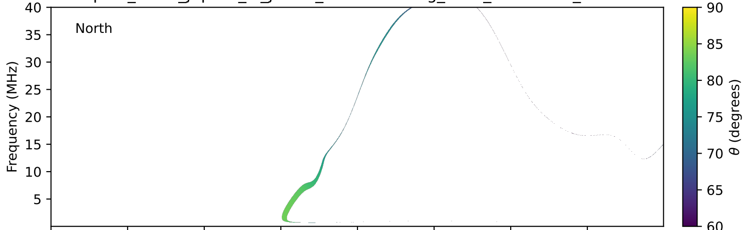
expres_earth_jupiter_io_jrm33_lossc-wid1deg_3kev_19770626_v11.cdf
