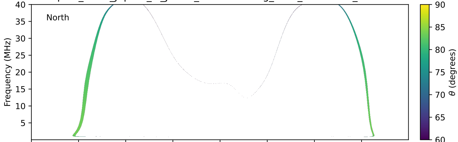
expres_earth_jupiter_io_jrm33_lossc-wid1deg_3kev_19770621_v11.cdf
