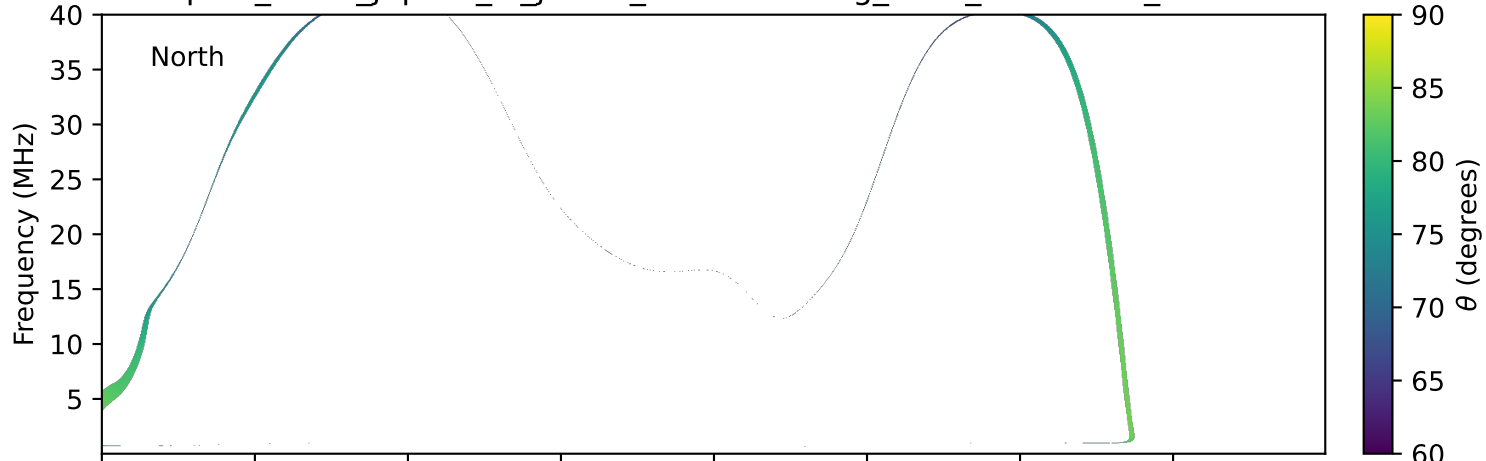
expres_earth_jupiter_io_jrm33_lossc-wid1deg_3kev_19770614_v11.cdf
