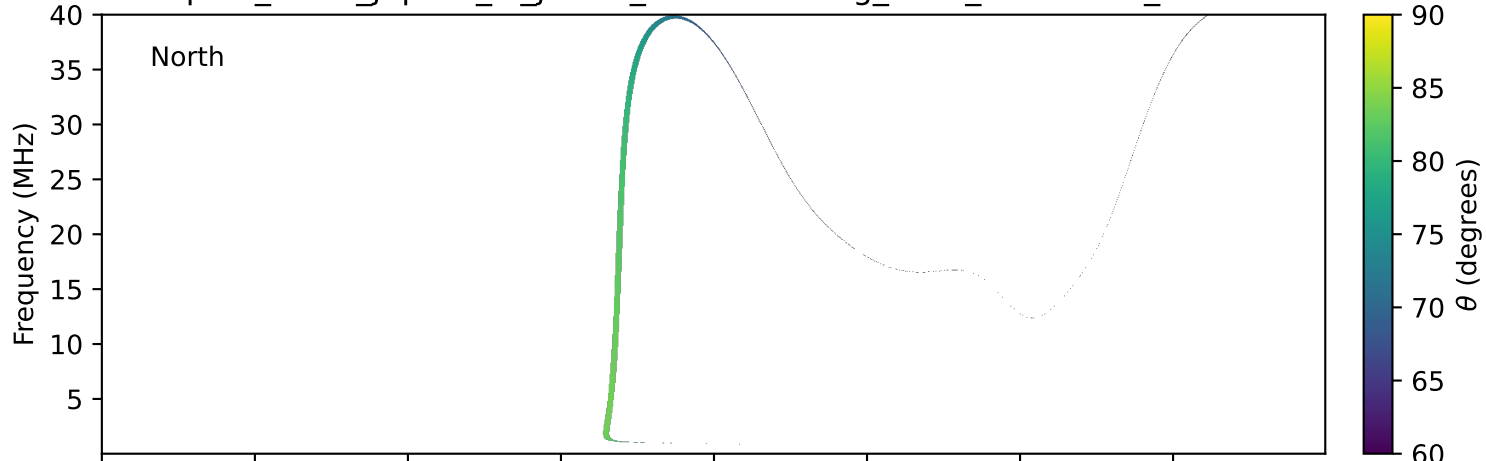
expres_earth_jupiter_io_jrm33_lossc-wid1deg_3kev_19770603_v11.cdf
