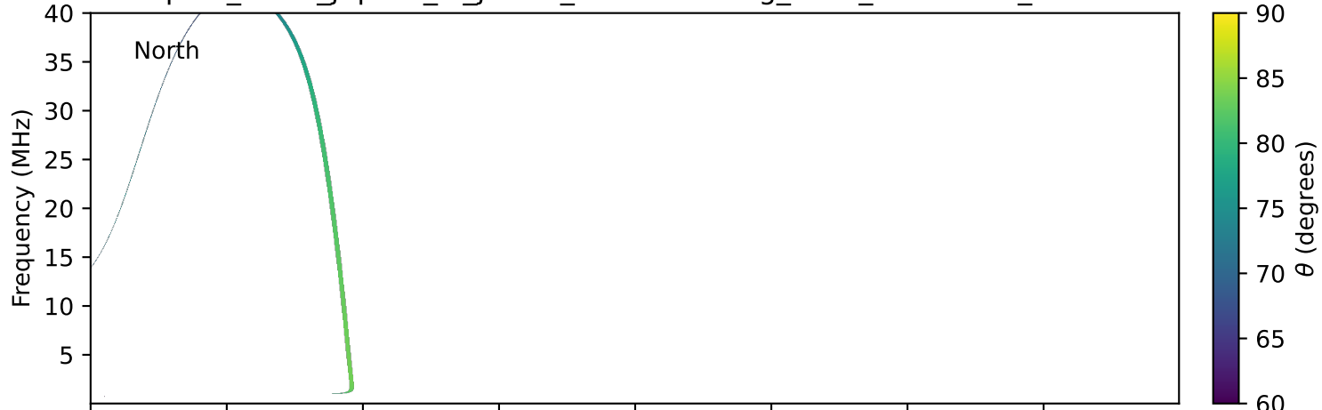
expres_earth_jupiter_io_jrm09_lossc-wid1deg_3kev_19770627_v11.cdf
