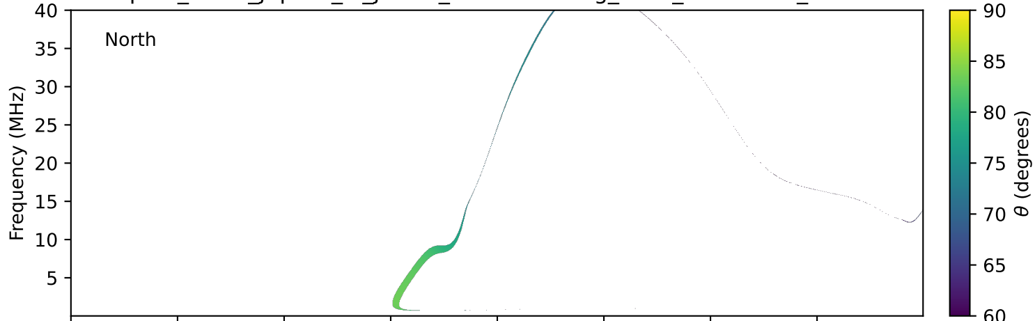
expres_earth_jupiter_io_jrm09_lossc-wid1deg_3kev_19770626_v11.cdf
