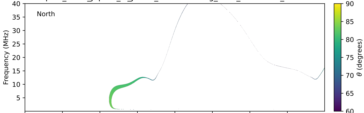
expres_earth_jupiter_io_jrm09_lossc-wid1deg_3kev_19770619_v11.cdf
