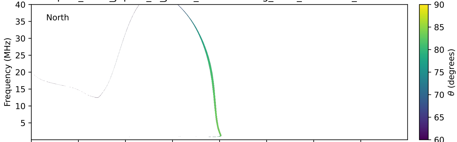
expres_earth_jupiter_io_jrm09_lossc-wid1deg_3kev_19770609_v11.cdf
