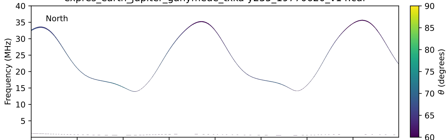
expres_earth_jupiter_ganymede_txka-y235_19770620_v14.cdf
