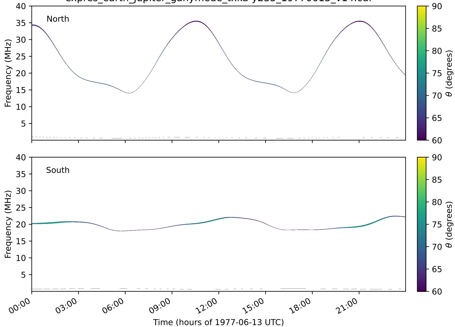
expres_earth_jupiter_ganymede_txka-y235_19770613_v14.cdf
