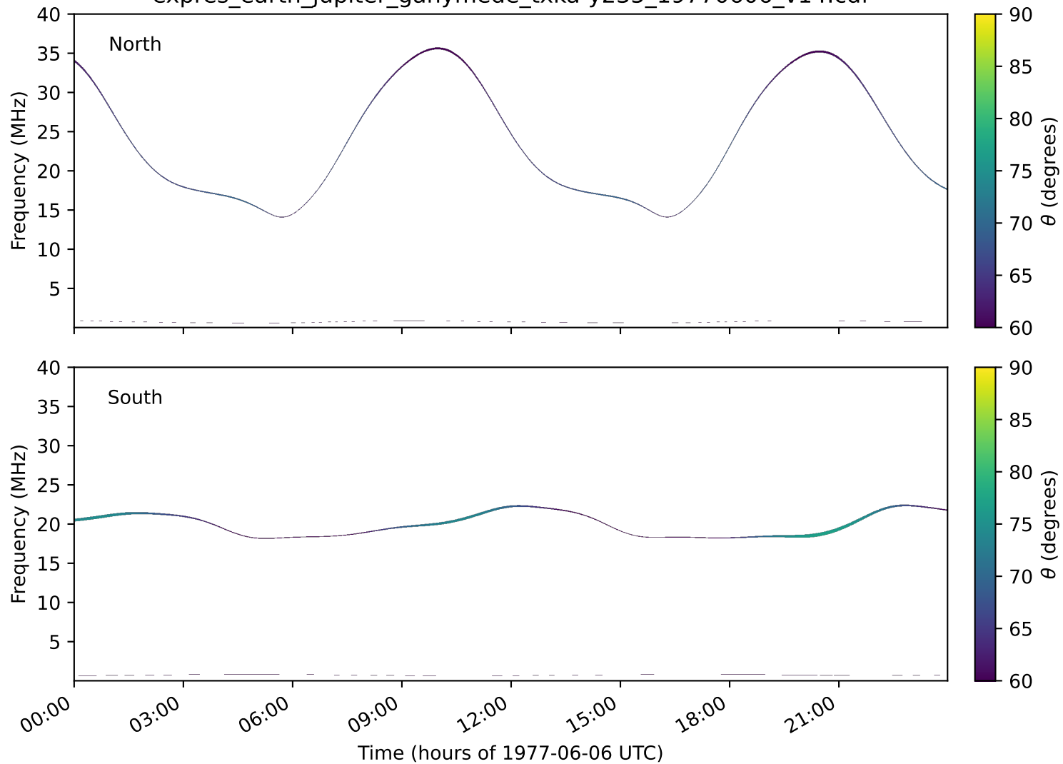
expres_earth_jupiter_ganymede_txka-y235_19770606_v14.cdf
