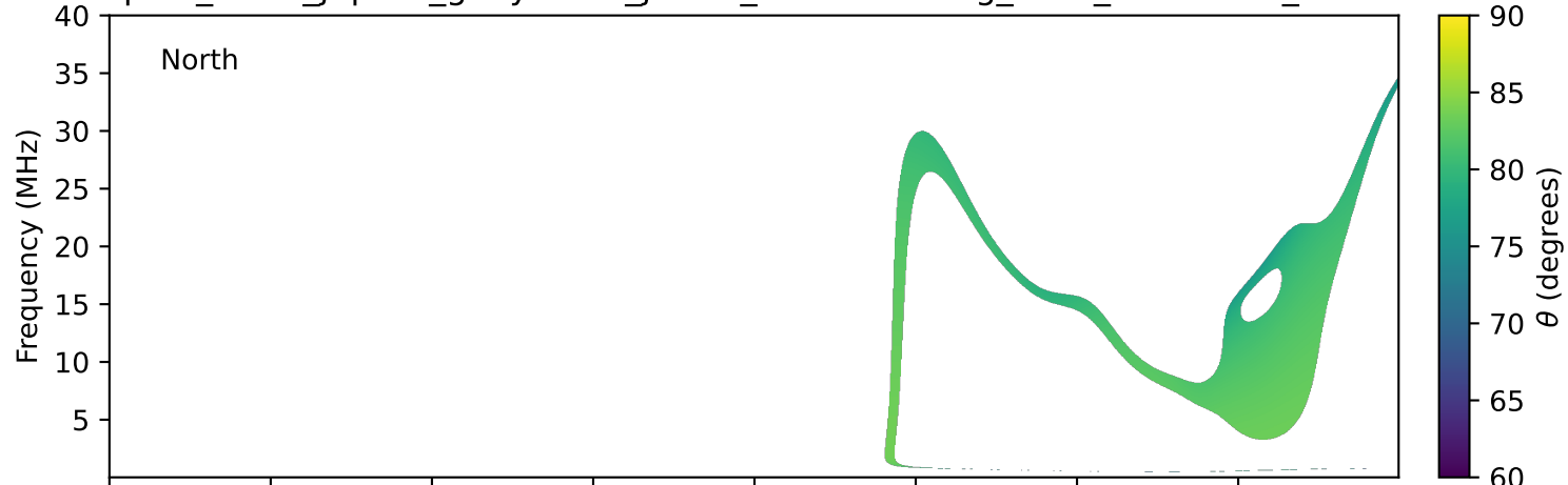
expres_earth_jupiter_ganymede_jrm33_lossc-wid1deg_3kev_19770626_v11.cdf
