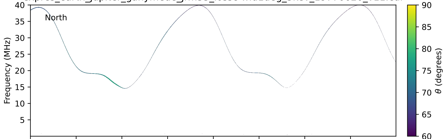
expres_earth_jupiter_ganymede_jrm33_lossc-wid1deg_3kev_19770620_v11.cdf
