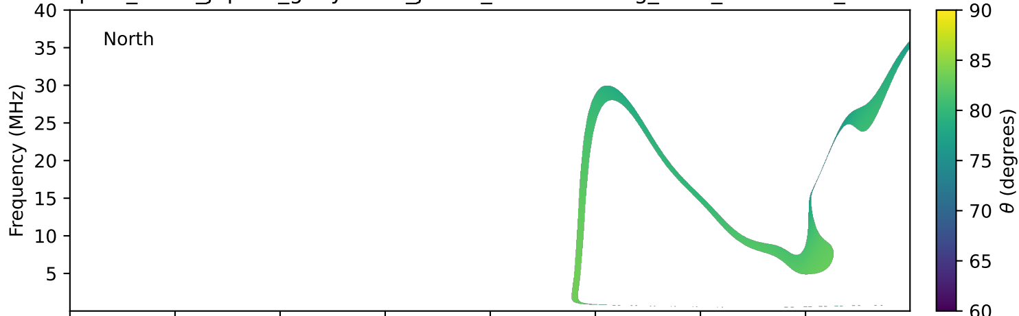
expres_earth_jupiter_ganymede_jrm09_lossc-wid1deg_3kev_19770626_v11.cdf
