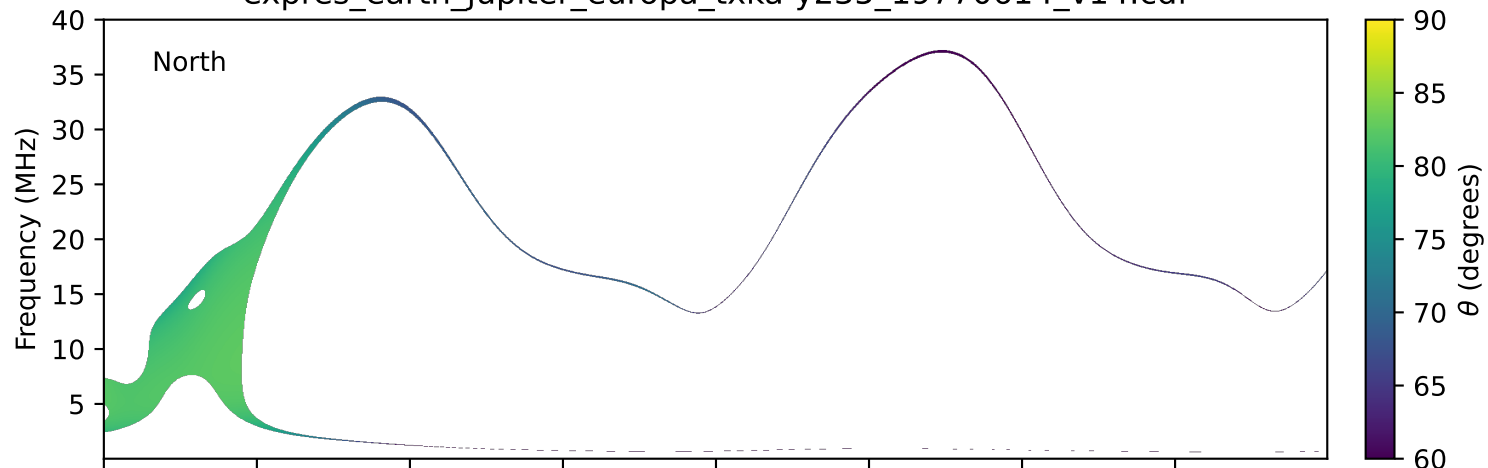
expres_earth_jupiter_europa_txka-y235_19770614_v14.cdf
