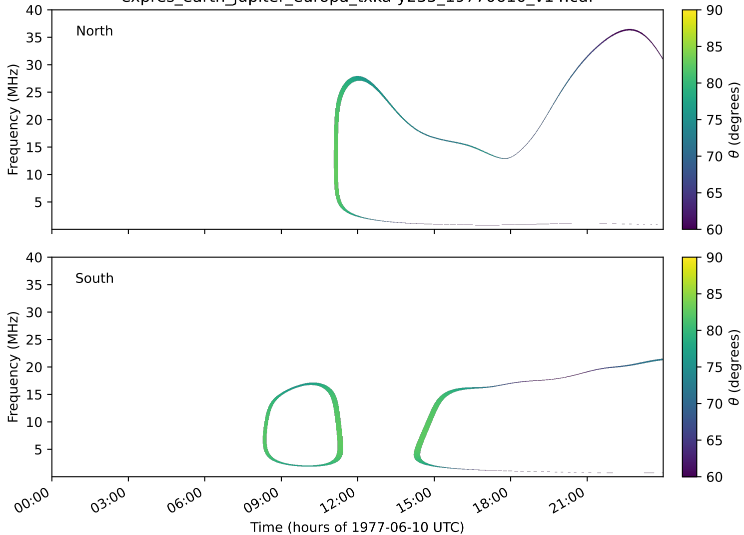
expres_earth_jupiter_europa_txka-y235_19770610_v14.cdf
