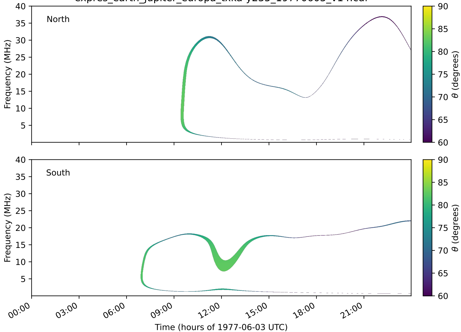
expres_earth_jupiter_europa_txka-y235_19770603_v14.cdf
