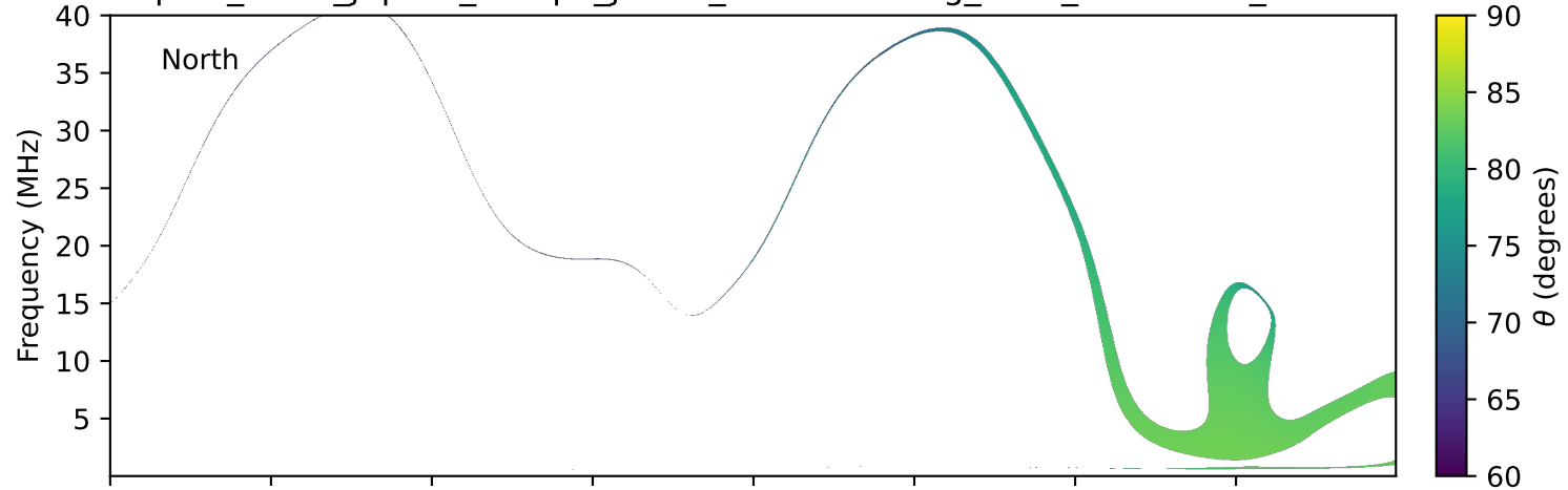
expres_earth_jupiter_europa_jrm33_lossc-wid1deg_3kev_19770629_v11.cdf
